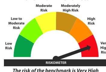
Benchmark Riskometer
